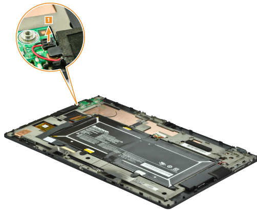
Figure 11. Removal steps of speakers
